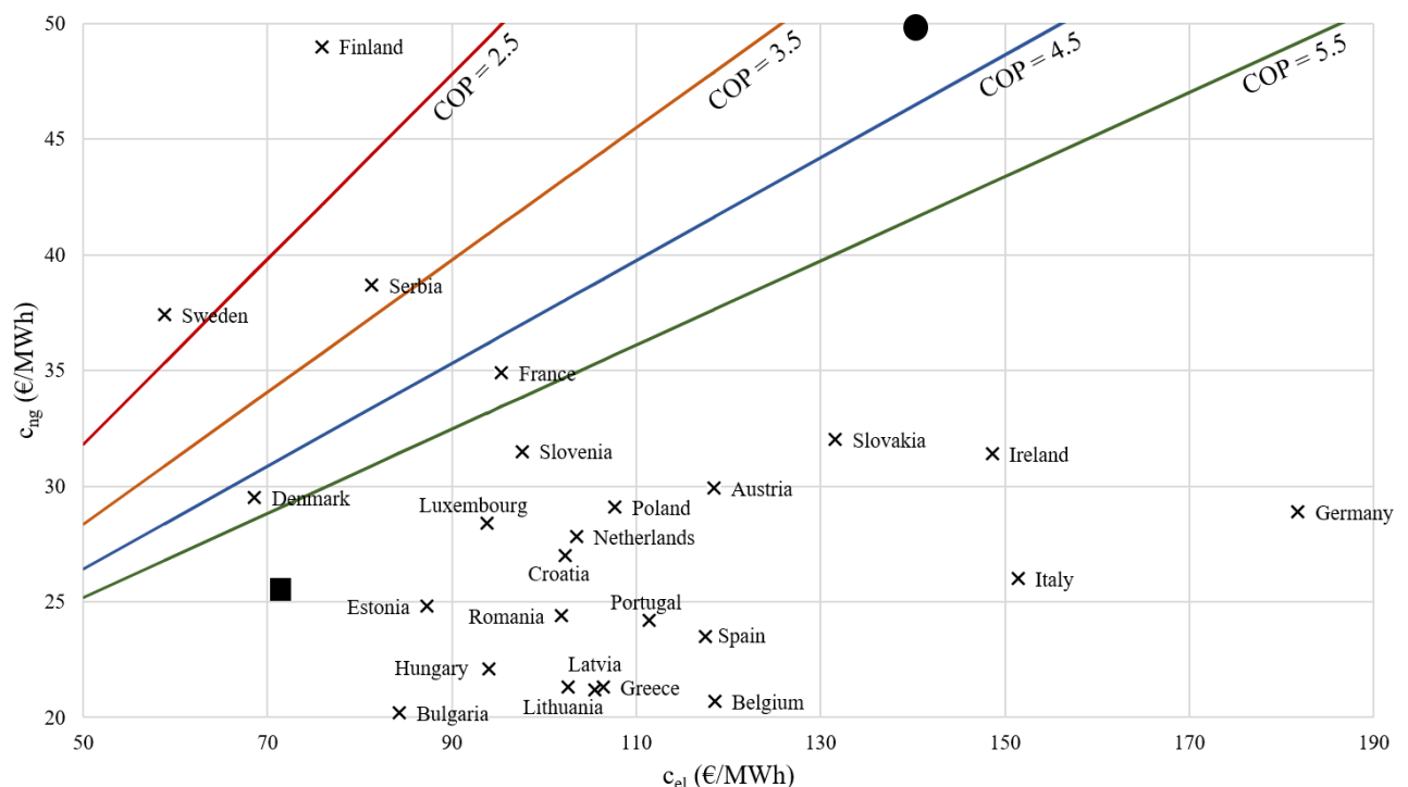
Fig. 37 - Positioning of European countries according to the gas price limits ( c_{ng,min} ) allowing the economic profitability for current COP range of MHPs. Coloured lines indicate the minimum gas cost ( c_{ng,min} ) that makes MHP cost-effective for a given COP. Cyprus, Malta, Czech Republic missing on the graph due to lack of economic data.
