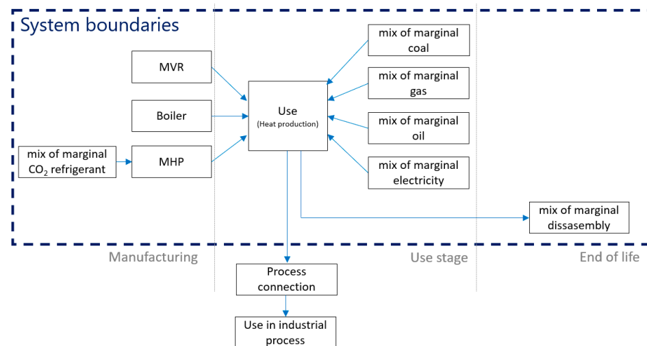
Figure A1. Flow diagram. The blue line indicates the system boundaries; all processes outside of the line are not considered in this study. The grey box represents the avoided energy consumption due to the change in the heat production system.
