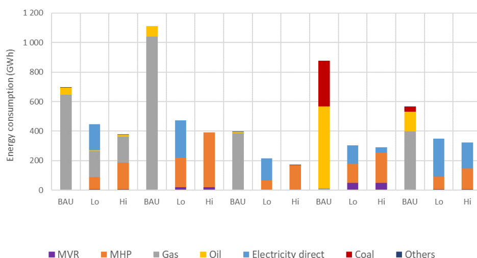
Fig. 1 – Danish food industry energy consumption by source
