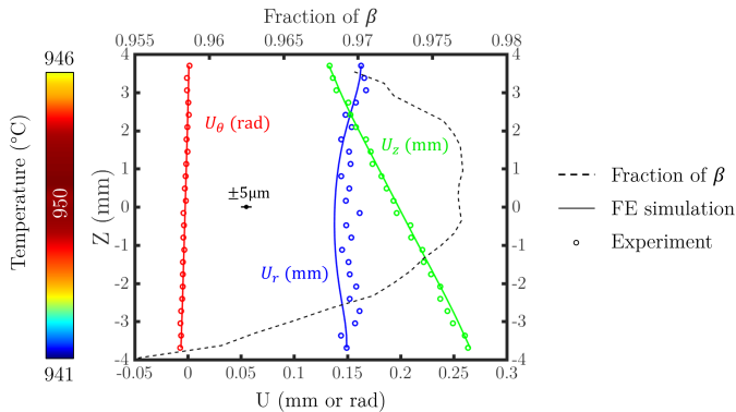
Figure 9: Comparison between the experimental and the numerical displacements obtained along an axial line at the middle of the ROI for the 9 bar test.
