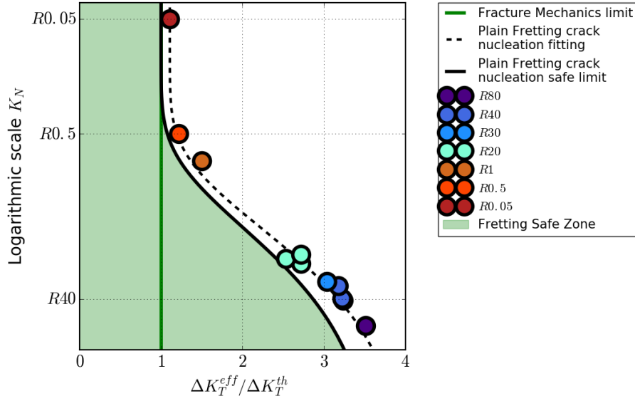
Figure 12 : Plain fretting crack nucleation prediction
